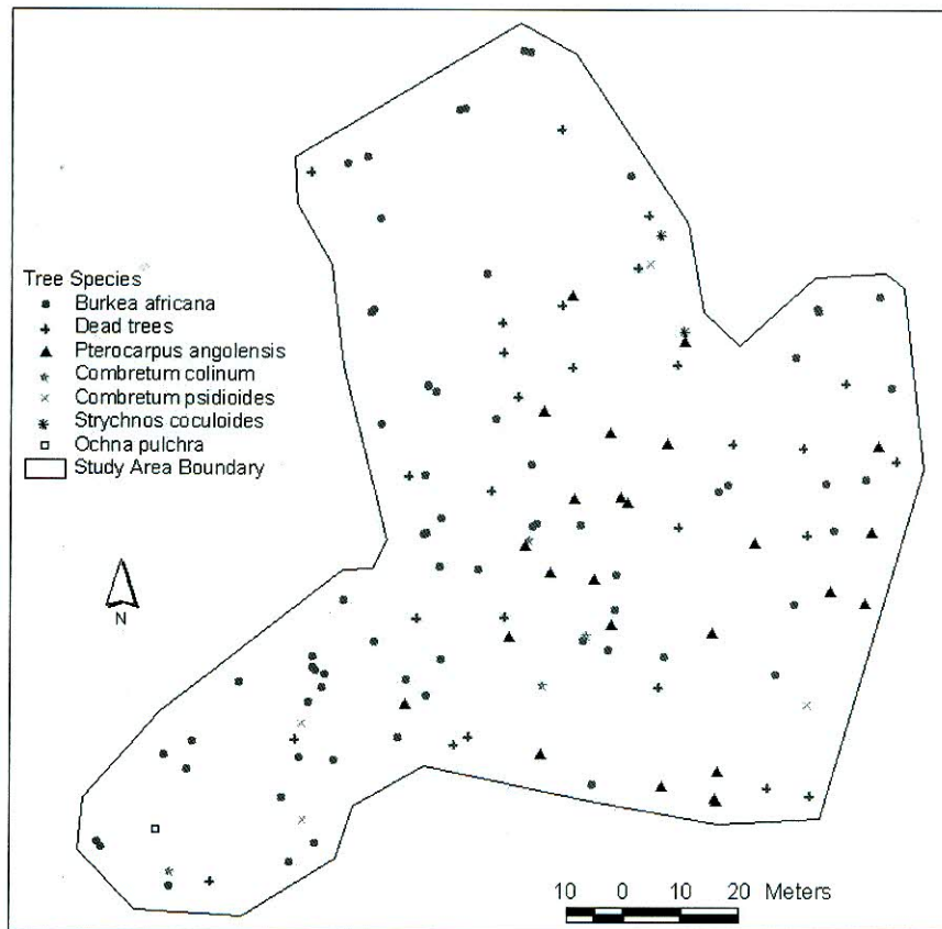
Figure 1: The dispersion of trees in a section of the dry savanna woodlands of northern Namibia.
